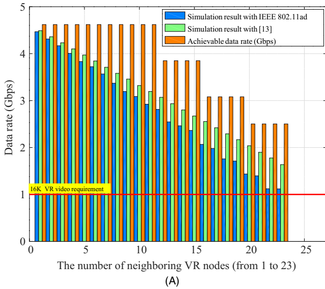
FIGURE 6 Simulation results for the data transfer rate and QoS satisfaction of the main stream in the deafness scenario; the number of neighboring nodes: 1 to 23; beamwidth is 30 degrees; r_{\max} denotes the transfer rate requirement of the user data. (A) Simulation results for data rate (more than 1 Gbps is required to support high-quality VR streaming data). (B) Quality estimation f_q(r) derived from achievable rate, r_{\max} = 1 Gbps for r_1 , r_{\max} = 2 Gbps for r_2 , and r_{\max} = 3 Gbps for r_3
