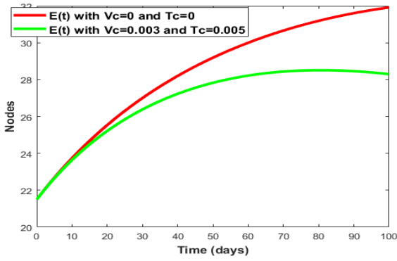
FIGURE 15. The time series plots of the node class E in an IoT system, as described by the system (67), with V_c = 0 , T_c = 0 and V_c = 0.003 , T_c = 0.005 .
