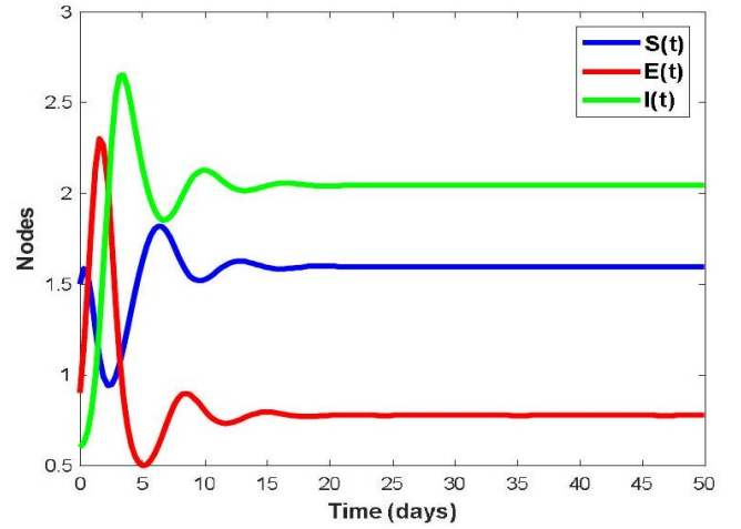
FIGURE 1. A time series plot of the node classes S(t) , E(t) and I(t) , derived from system (67), with \tau = 0 .
